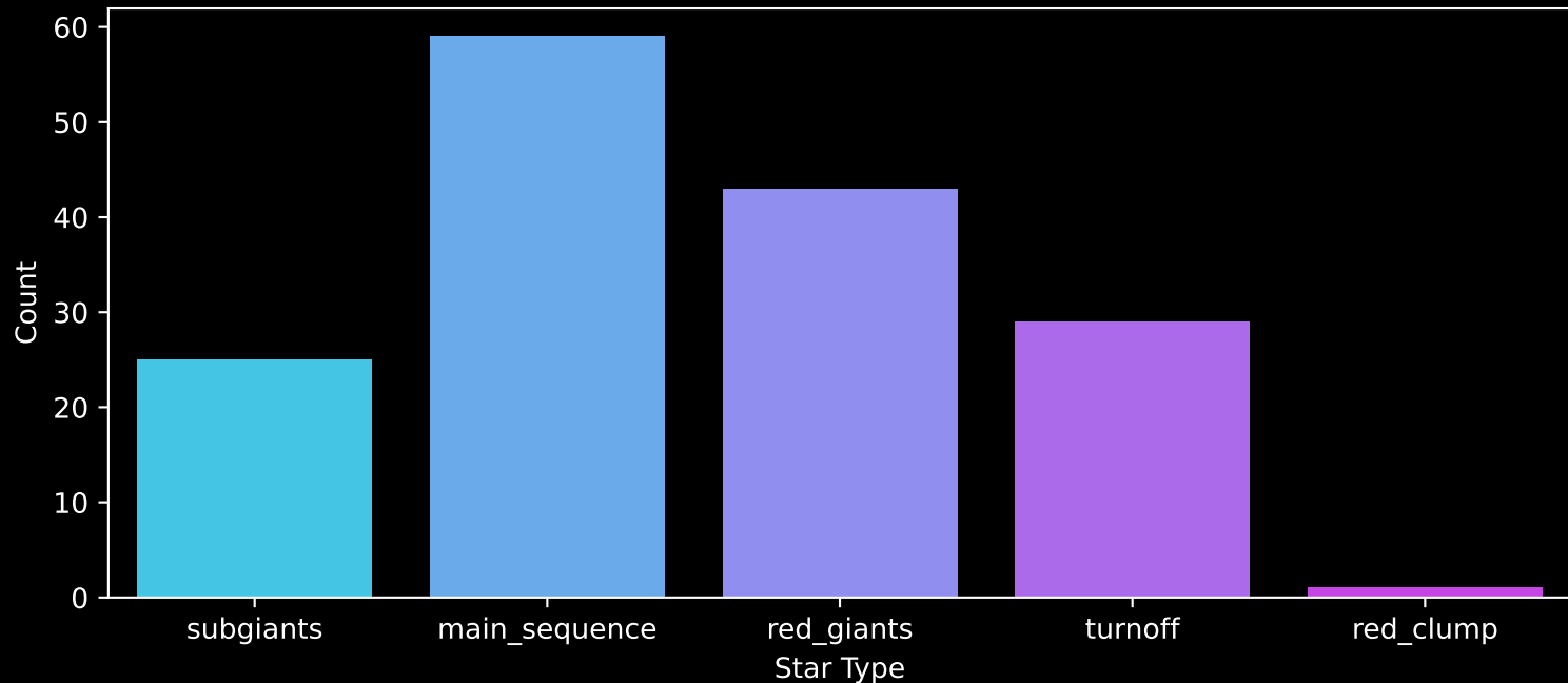
APOGEE DR17 Field: [LMC28] Count plot of Star Type
