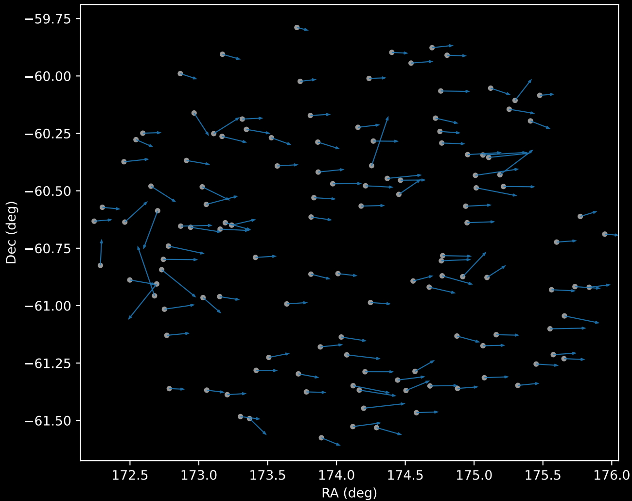
APOGEE DR17 Cluster 0 Proper Motion Vectors (n=128)
