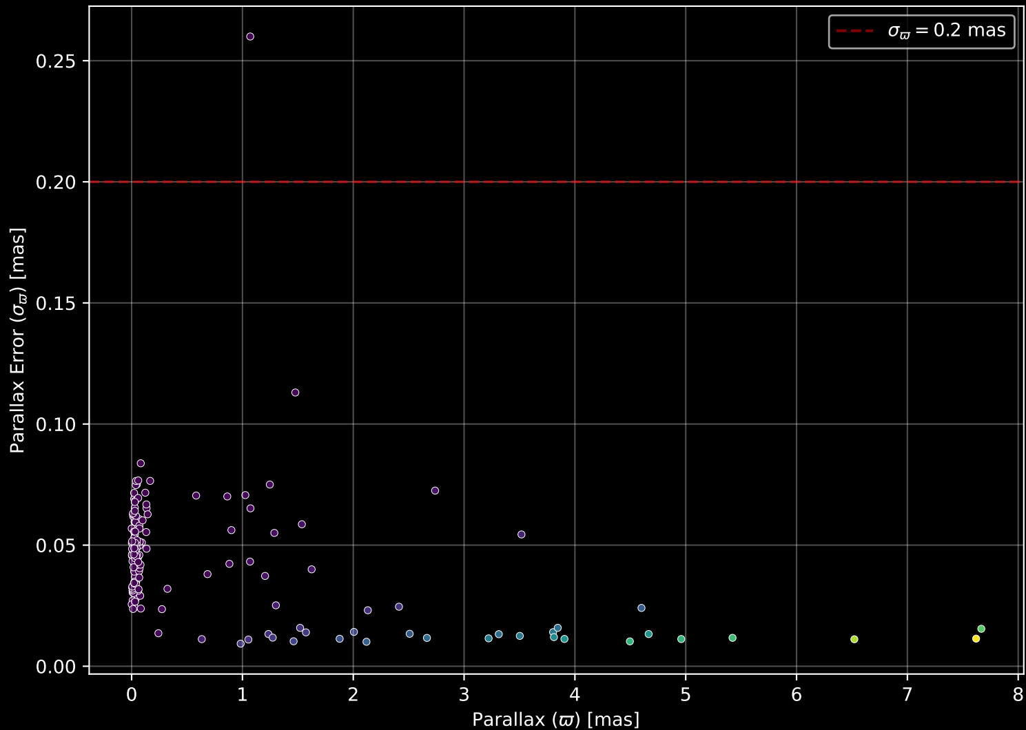
APOGEE DR17 Field: [LMC28] Parallax Quality (n= 157)
