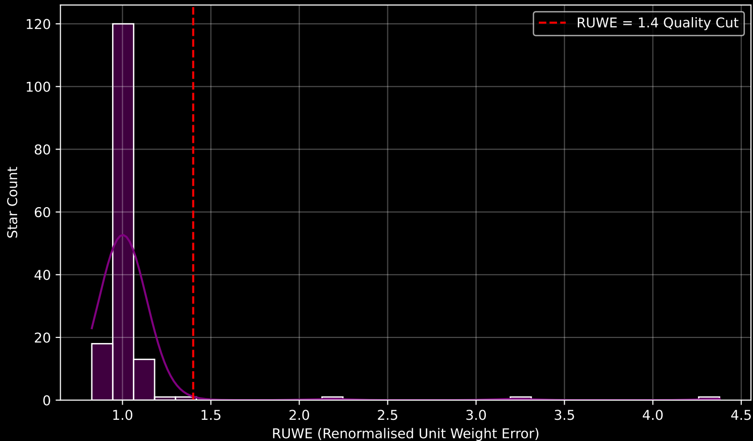
GAPOGEE DR17 Field [LMC28] RUWE Distribution (n= 156)
