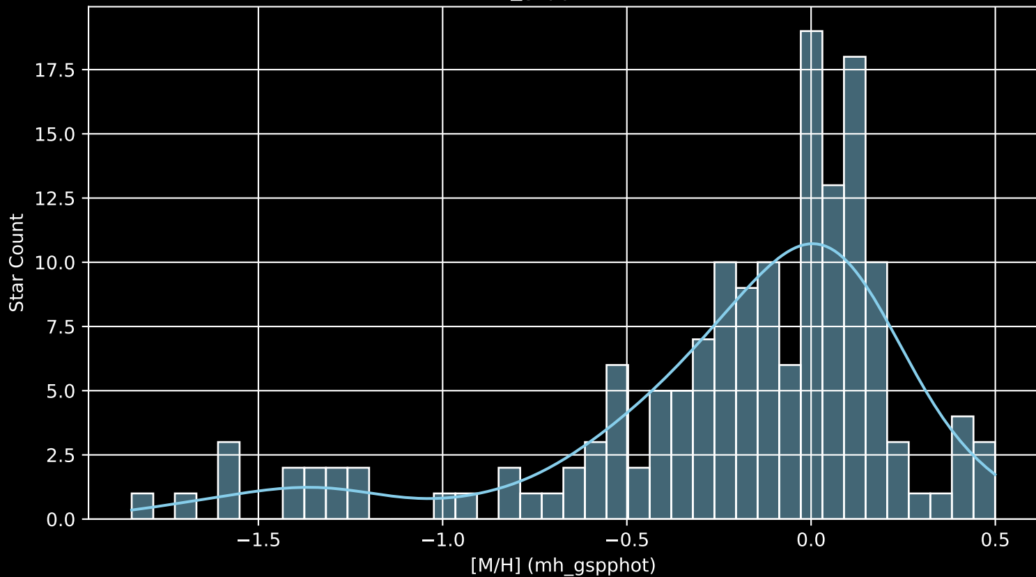
APOGEE DR17 Field: [LMC28 [M/H] (mh_gspphot) (n= 156)
