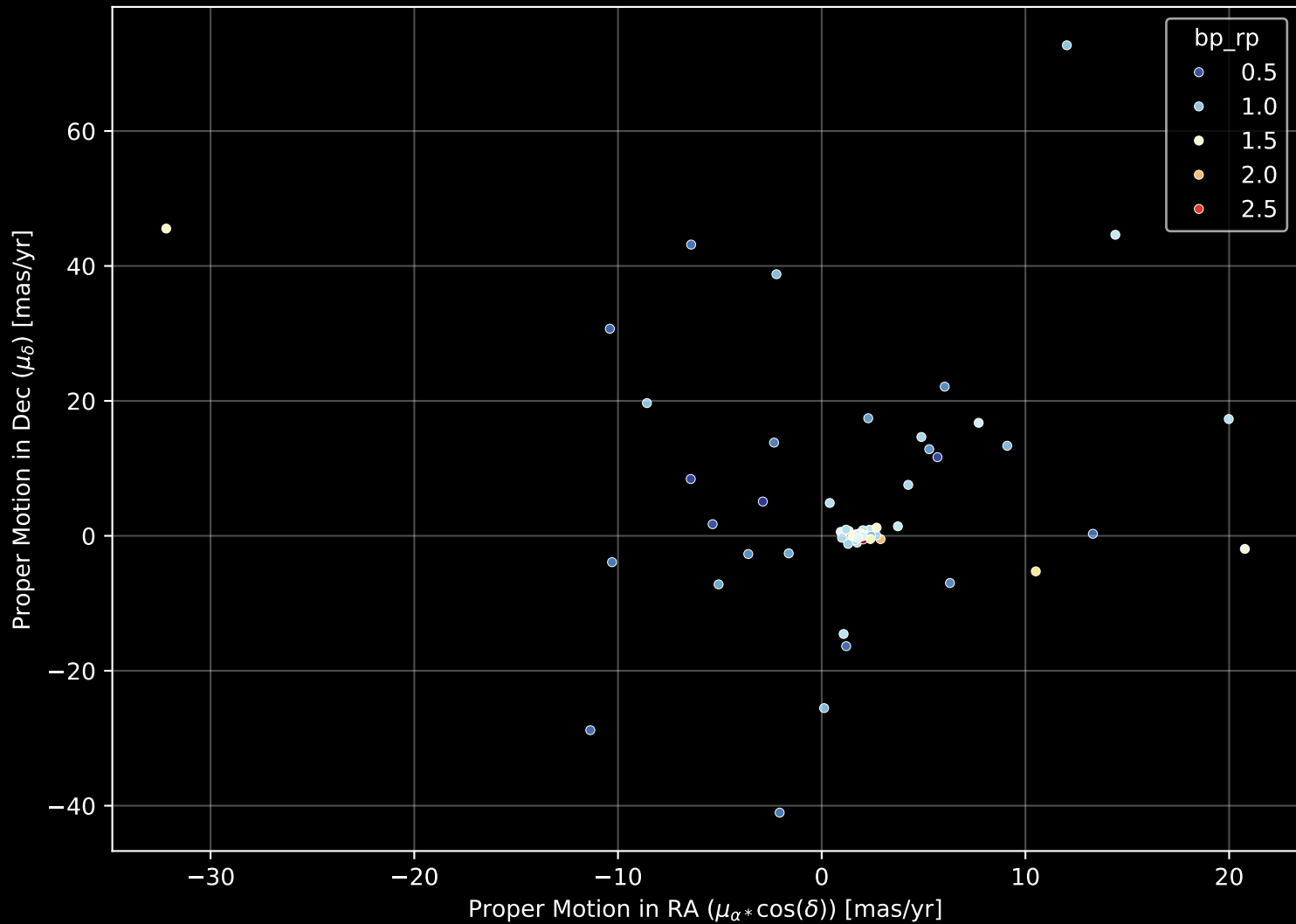
APOGEE DR17 Field: [LMC28] Proper Motion Diagram (n= 157)
